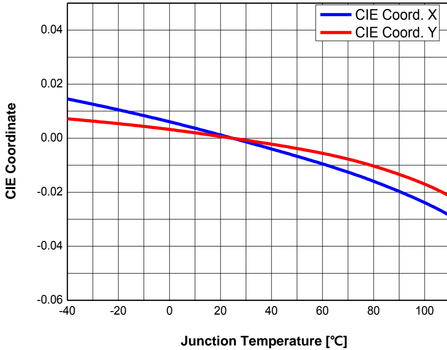
Fig 8. Chromaticity Coordinate vs. Junction Temperature, I_F = 20\text{mA}
